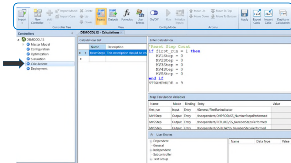
Figure: Screenshot of DMC3 Builder Controllers navigation tree, Calculations section
